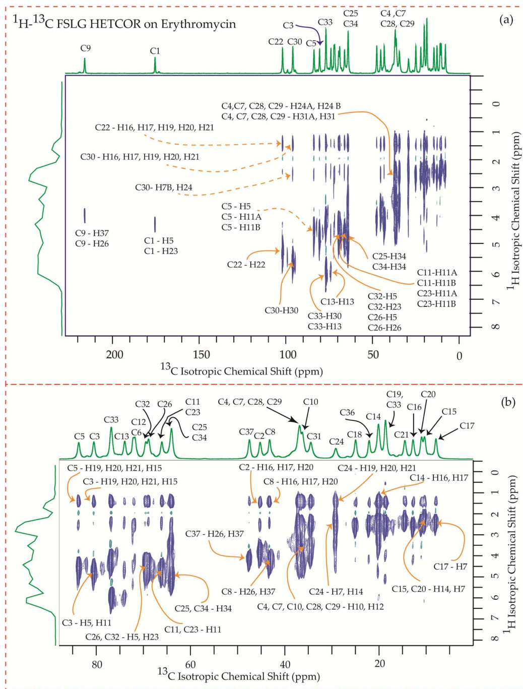
Fig. 23 (a) ^1\text{H} - ^{13}\text{C} FSLG HETCOR spectrum of erythromycin. (b) Enlarged version of ^1\text{H} - ^{13}\text{C} FSLG HETCOR spectrum from C5 to C17.
