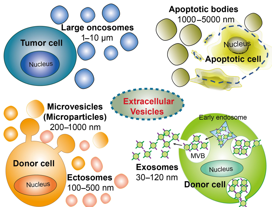
Figure 1 Schematic representation of the EV biogenesis. EVs family has more than four members, they are exosomes (30–120 nm), microparticles (or microvesicles, 200–1000 nm), ectosomes, 100–500 nm), large oncosomes (1–10 \mu\text{m} ), and apoptotic bodies (1–5 \mu\text{m} ).
