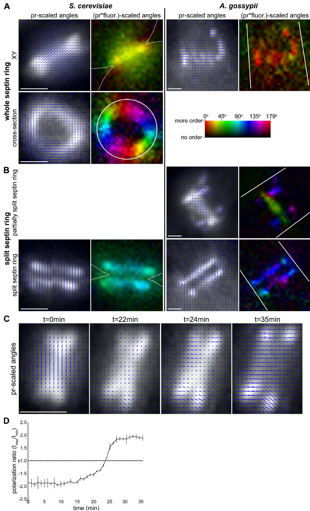
Figure 4. Septin rings in S. cerevisiae and A. gossypii are similarly ordered and accomplish a \approx 90^\circ change in orientation without concerted rotation. (A) Septin rings assembled in S. cerevisiae and A. gossypii expressing Cdc12-conGFP4 exhibit septins organized such that, on average, GFP dipoles are oriented perpendicular to the cell growth axis. As in A. gossypii (Fig. 3C), the S. cerevisiae septin hourglass, when viewed in cross section, also has the average GFP dipole position oriented parallel to the cell cortex, and perpendicular to the growth axis. Cell outlines are shown in white. Bars, 1 \mu\text{m} .
