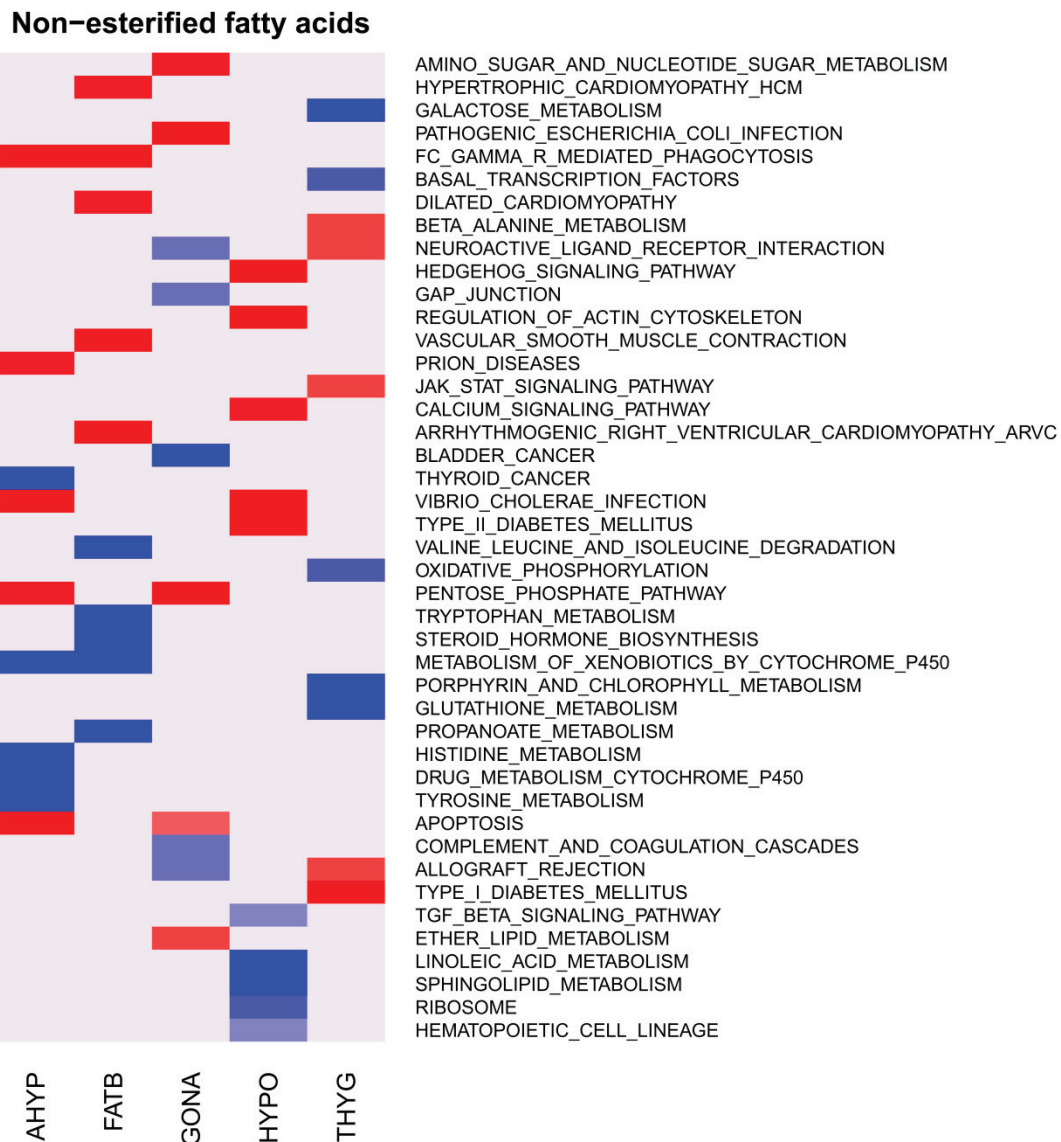
Figure 2 Heat map of KEGG pathways enrichment scores for non-esterified fatty acids in five tissues. Red (blue) denotes top five pathways with positive (negative) normalized enrichment scores in gene set enrichment analysis (GSEA) for backfat (FATB), gonad (GONA), adenohipophys (AHYP), thyroid (THYG), hypothalamus (HYPO).
