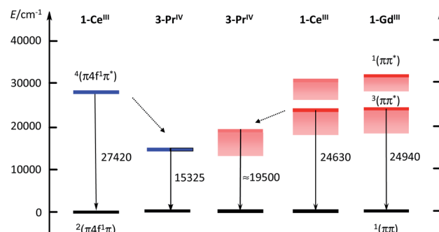
Fig. 6 Partial electronic diagram for 1-Ce, 3- \text{Pr}^{\text{MeCN}} , and 1-Gd. Calculated levels in blue, experimental 0-phonon levels in red or rose when estimated from the onset of the emission band. Energies of the transitions in \text{cm}^{-1} .
