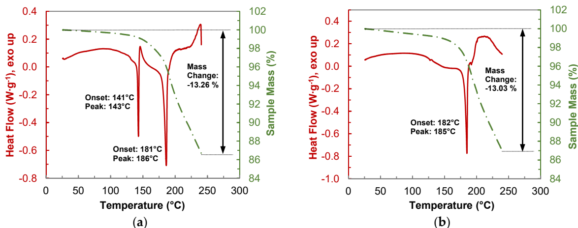
Figure 12. Thermogravimetric analysis (TGA-DSC) of (a) a 1:1 physical mixture of BDMC and HYQ, (b) BDMC-HYQ co-crystal produced by LAG; heating rate: 2 °C·min -1 .
