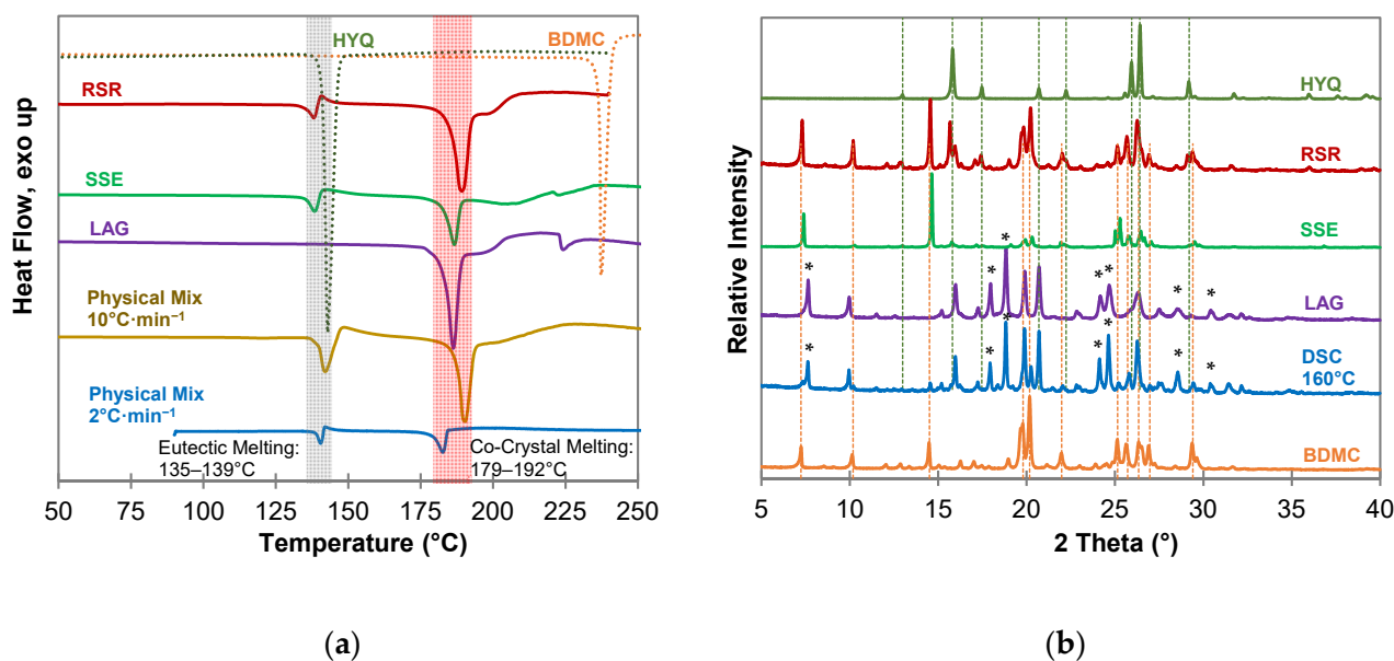
Figure 6. Characterization of BDMC, HYQ, and co-crystallization products of BDMC and HYQ, (a) DSC thermograms at a heating rate of 10\text{ }^{\circ}\text{C}\cdot\text{min}^{-1} and 2\text{ }^{\circ}\text{C}\cdot\text{min}^{-1} (blue line): DSC curves of pure substances are shown as dotted lines, grey bar indicates eutectic melting, red bar indicates co-crystal melting; (b) PXRD diffractograms: characteristic peaks of pure HYQ and BDMC are marked as dotted green and orange lines, * new diffraction peaks; abbreviations: RSR-rapid solvent removal, SSE-slow solvent evaporation, LAG-liquid assisted grinding, DSC-differential scanning calorimetry.
