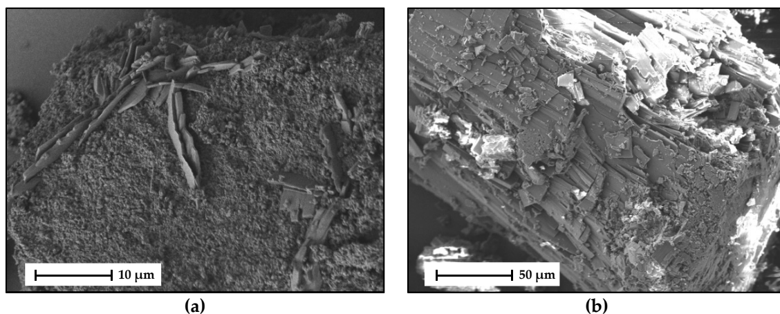
Figure 15. SEM micrographs of (a) HYQ-BDMC co-crystals produced by LAG at 2500 \times magnification, (b) HYQ-BDMC co-crystals produced by slow solvent evaporation from toluene/ethyl acetate (50/50 v/v ) at 500 \times magnification; (a) detection of back scatter electrons; (b) detection of secondary electrons.
