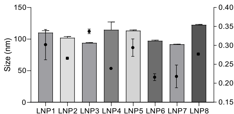
Figure 1 Synthesis and characterization of lipid nanoparticles (LNPs) for pDNA delivery in cardiomyocytes. (A) Left: LNPs were formulated via microfluidic mixing of an aqueous phase of pDNA and an ethanol phase of lipids. Right: Schematic formation of LNPs encapsulating pDNA (Right). (B) Hydrodynamic diameter measurements and polydispersity index of LNPs. Bar graph: size; Bar dot: PDI (polydispersity index). (C) Representative cryo-TEM of LNPs encapsulating pDNA. Data are plotted as mean \pm SEM.
