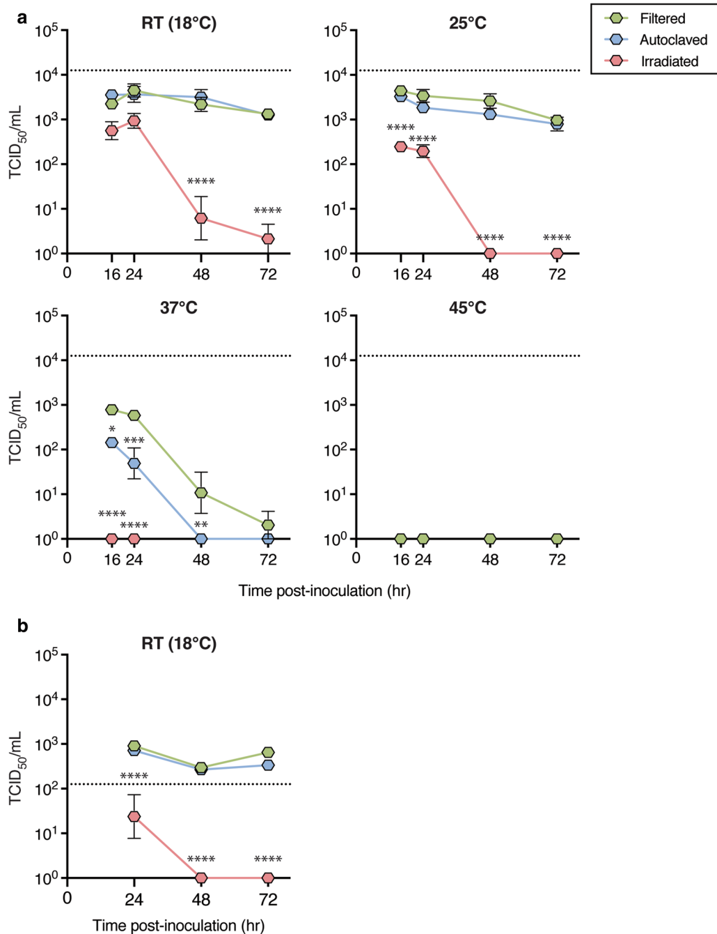
Fig. 2 Preservation of viral infectivity in samples varies with VTM sterilization method and is affected by storage temperature and starting dose. VTM sterilized by filtration, autoclave or irradiation was inoculated at a level of a 1.2 \times 10^4 TCID 50 /mL or b 1.2 \times 10^2 TCID 50 /mL SARS-Cov-2, and then incubated at indicated temperatures for up to 72 h. Shown are mean \pm SEM for 5–7 data points, pooled from two independent experiments. Dashed lines represent the final concentration of virus used to inoculate the VTM. Two-way ANOVA with Tukey’s post-tests was used to compare all groups at each time point; * indicates any group that showed a p value less than 0.05 compared to the filtered group, * p < 0.05, ** p < 0.01, *** p < 0.001, **** p < 0.0001
