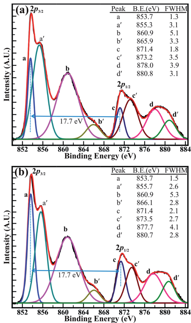
Fig. 5 High-resolution XPS spectra of the Ni (2p) core levels of the Ni-oxides decomposed at a temperature of (a) 500 °C and (b) 700 °C. The XPS spectra were decomposed using Voigt peak function fittings.
