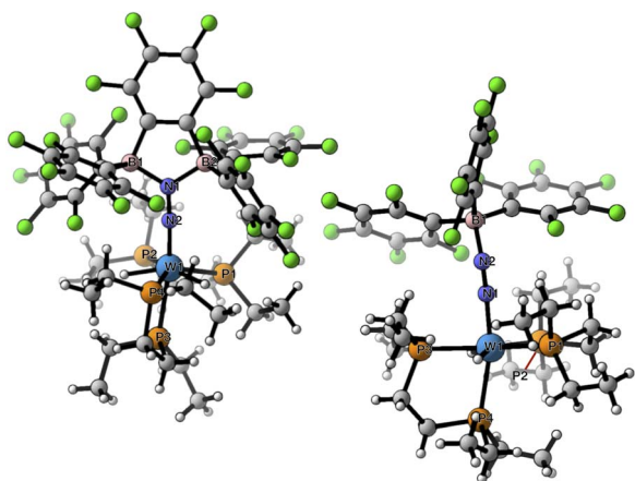
Fig. 4 Molecular structures of complexes 7 (left) and 10 (right) in the solid state. Selected distances ( \text{\AA} ) and angles ( ^\circ ): 7: W1–P1 2.559(1), W1–P2 2.516(1), W1–P3 2.651(1), W1–P4 2.475(1), W1–N2 1.825(2), N1–N2 1.291(3), N1–B1 1.615(3), N1–B2 1.614(3), W1–H100 1.66(3), W1–H200 1.62(2), W1–N2–N1 177.0(2), N2–N1–B1 125.0(2), N2–N1–B2 121.8(2), B1–N1–B2 113.3(2). 10: W1–P1 2.4813(5), W1–P2 2.4792(5), W1–P3 2.4300(5), W1–P4 2.5214(5), W1–N1 1.8826(17), N1–N2 1.193(2), N1–B1 1.562(3), W1–H1 1.71(3), W1–H2 1.70(3), W1–N1–N2 167.21(15), N1–N2–B1 139.13(18).
