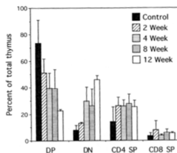
Figure 2. Anti-IL-7 treatment alters the proportion of CD4- and CD8-defined thymic subsets. Thymic cells were obtained from mice treated for 2–12 wk and processed for flow cytometry as described in Materials and Methods. The cells were stained with PE-conjugated anti-CD4 and Cyanine-conjugated anti-CD8 before flow cytometric analysis. The percentage of each population was calculated by integration. The control group represents the average of all mice injected with the isotype-matched mouse IgG. The values present the mean (three–five mice per group) \pm SEM.
