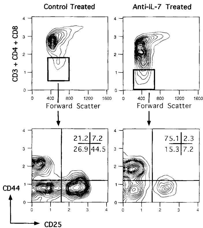
Figure 5. TN thymocytes become IL-7 responsive at the CD44 + , CD25 + stage. Thymocytes from mice treated for 4 wk with anti-IL-7 or control IgG were stained with PE-conjugated antibodies to CD3, CD4, and CD8, Cyanine conjugated anti-CD25, and FITC-conjugated anti-CD44. The TN population was gated as shown ( top ), to reveal the CD44 + and CD25 + defined subsets within this compartment. The CD3 - , CD4 - , CD8 - gate in the anti-IL-7-treated mouse was set lower to eliminate the large proportion of the CD3 lo , DN TCR \alpha, \beta + cells. CD25 + cells were not eliminated due to the lower gating. The values refer to the percentage of cells within each quadrant of the TN compartment.
