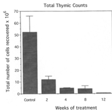
Figure 1. Thymic cell recovery is markedly decreased by the administration of anti-IL-7 antibody. Cell counts were obtained from the suspended thymus glands of adult BALB/c mice (three–five per group) intraperitoneally injected with 1 mg of monoclonal anti-IL-7 antibody three times a week for 2, 4, 8, or 12 wk. The control group represents the mean of all mice similarly injected with the isotype matched mouse IgG. (12-wk control-treated thymus averaged 58 \times 10^6 recovered cells). The data are shown as mean \pm SEM.
