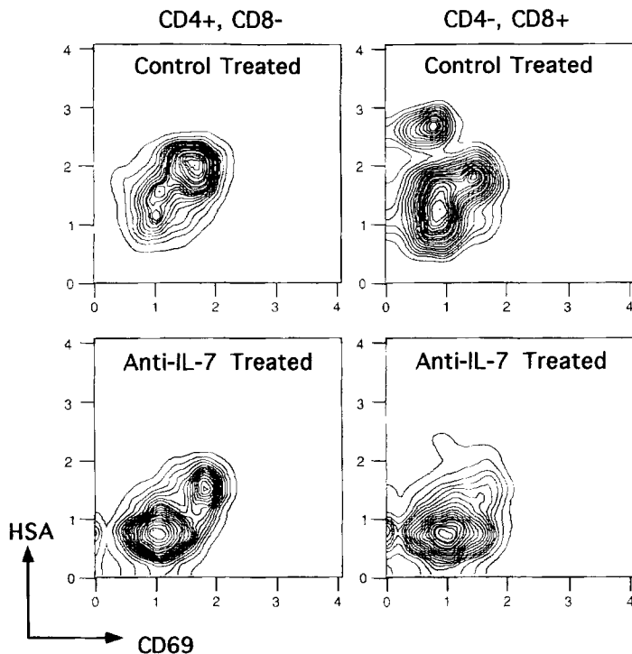
Figure 6. Anti-IL-7 treatment markedly reduces thymocytes undergoing selection events. Thymocytes from mice treated for 4 wk with M25 or control IgG were stained with PE-conjugated anti-CD4, Cyanine-conjugated anti-CD8, FITC-conjugated anti-HSA, and biotin-conjugated anti-CD69 plus Texas Red-avidin. The CD69 vs. HSA contours are derived from the CD4 + , CD8 - and CD4 - , CD8 + gated populations.
