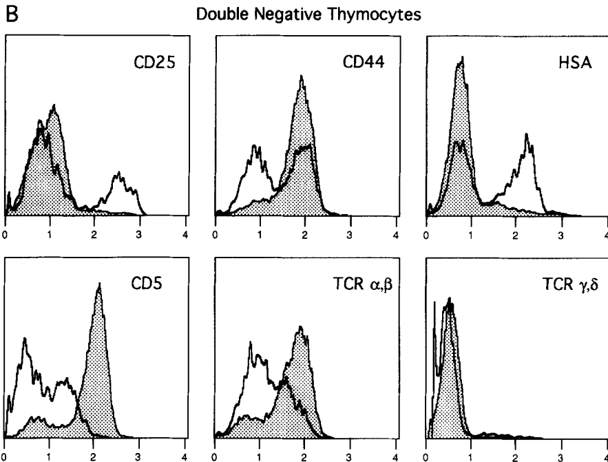
Figure 3. Anti-IL-7 treatment depletes a DN CD25+, CD44-, HSA+, CD5-, TCR \alpha,\beta + subset. Thymic cells from adult BALB/c mice treated for 8 wk with anti-IL-7 or isotype-matched control antibody were stained with conjugated antibodies and analyzed by three-color flow cytometry as described in Materials and Methods. Cells were stained with PE-conjugated anti-CD4, Cyanine-conjugated anti-CD8, and biotin-conjugated antibodies to CD25, CD44, HSA, CD5, TCR \alpha,\beta , or TCR \gamma,\delta plus FITC-avidin. (A) Two-color contours of CD4- and CD8-stained thymocytes. (B) Phenotype of CD4-, CD8- gated thymocytes from anti-IL-7 (shaded histograms)- and control IgG (open histograms)-treated mice. In A, the percentages for the DN, DP, CD4 SP, and CD8 SP subsets are shown to the right of each contour plot.
