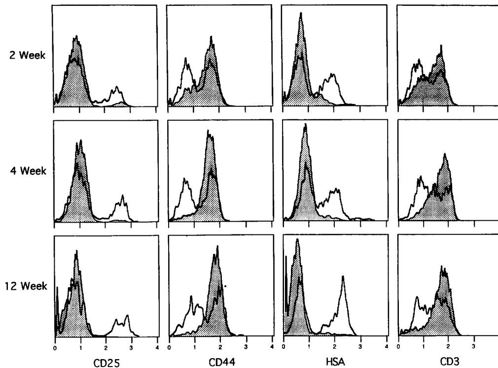
Figure 4. Early thymocytes are progressively lost with anti-IL7 treatment. Thymocytes from mice treated with M25 for 2, 4, and 12 wk ( shaded histograms ) or mice similarly treated with control antibody ( open histograms ) were stained with PE-conjugated anti-CD4, Cyanine-conjugated anti-CD8, and biotin-conjugated antibodies to CD25, CD44, HSA, CD5, or CD3 plus FITC-avidin. The histograms are derived from the CD4 - , CD8 - gated populations.
