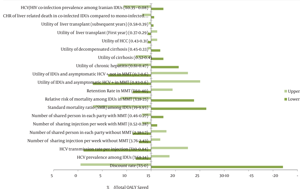
Figure 2. Results of One-Way Sensitivity Analysis (Tornado Diagram)
