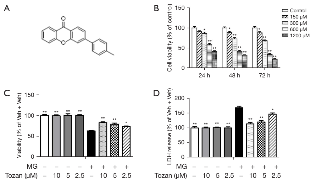
Figure 1 Tozan ameliorates cell damage caused by MG. (A) The structure of Tozan. The compound structure was confirmed by ^1\text{H} NMR and ^{13}\text{C} NMR, details as follows: M. P. 127–128 ^{\circ}\text{C} ; ^1\text{H} NMR (500 MHz, \text{CDCl}_3 ) \delta (ppm) 8.35–8.32 (m, 2H), 7.71–7.68 (m, 1H), 7.63 (d, J = 1.5 Hz, 1H), 7.58–7.55 (m, 3H), 7.46 (d, J = 8.5 Hz, 1H), 7.36 (t, J = 7.5 Hz, 1H), 7.28 (d, J = 8.0 Hz, 2H), 2.40 (s, 3H); ^{13}\text{C} NMR (125 MHz, \text{CDCl}_3 ) \delta (ppm) 176.9, 156.4, 156.2, 147.7, 138.8, 136.2, 134.6, 129.7, 127.4, 127.1, 126.6, 123.8, 122.7, 121.9, 120.3, 117.9, 115.4, 21.2. (B) Effect of MG on the survival rate of SH-SY5Y cells at different doses and different times. Cell viability was assessed by the MTT method. Results are shown as means \pm SEM ( n=6 ). * P < 0.05 , ** P < 0.01 vs. control group. (C,D) Tozan increased the survival rate of MG-induced cells as determined by the MTT method and decreased the LDH release of MG-induced SH-SY5Y cells. Data are shown as means \pm SEM ( n=6 ). * P < 0.05 , ** P < 0.01 vs. MG + Veh group. MG, methylglyoxal; SEM, standard error of mean.
