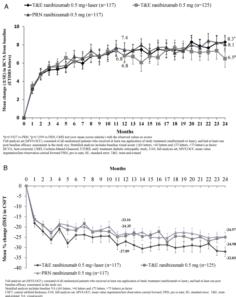
Figure 2 (A) Mean change in best-corrected visual acuity (BCVA) from baseline to months 12 and 24 (full analysis set (FAS)-mean value imputation/last observation carried forward (MV/LOCF)). * p=0.9327 versus pro re nata (PRN); # p=0.1599 versus PRN; Cochran–Mantel–Haenszel (CMH) test (row mean scores statistic) with the observed values as scores. (B) Mean percentage change in central subfield thickness (CSFT) from baseline over time (FAS-MV/LOCF). In (A) and (B), FAS (MV/LOCF) comprised all randomised patients who received at least one application of study treatment (ranibizumab or laser) and had at least one postbaseline efficacy assessment in the study eye. Stratified analysis included baseline visual acuity ( \leq 60 letters, >60 and \leq 73 letters and >73 letters) as factors. ETDRS, Early Treatment Diabetic Retinopathy Study.
