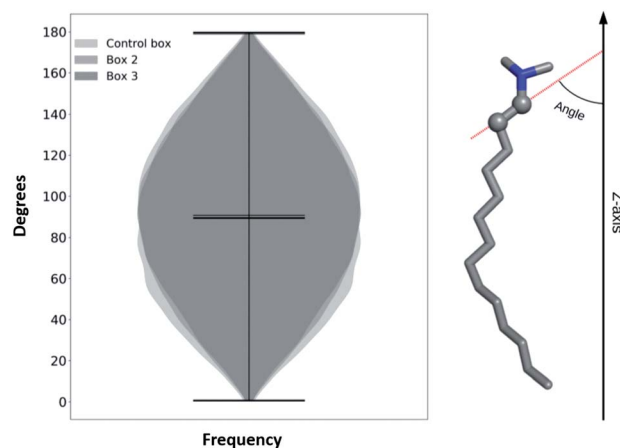
Fig. 5 Histogram of a characteristic inner angle of a TTA + 's when are in the bulk solution of Box 2, Box 3 and from 1 TTA + in water for 200 ns.
