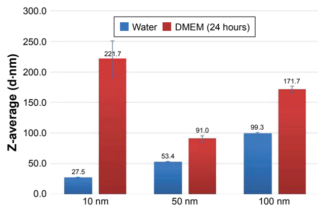
Figure 1 Z-average hydrodynamic size of 10, 50, and 100 nm silver nanoparticles diluted with water and DMEM cell-cultured media (24 hours).
