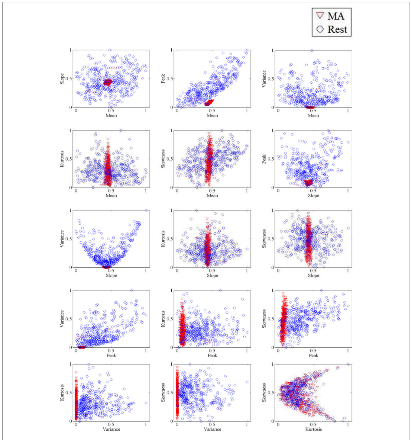
FIGURE 2 | The 2-dimensional feature spaces of Subject 1 for all combinations of HbO features.
