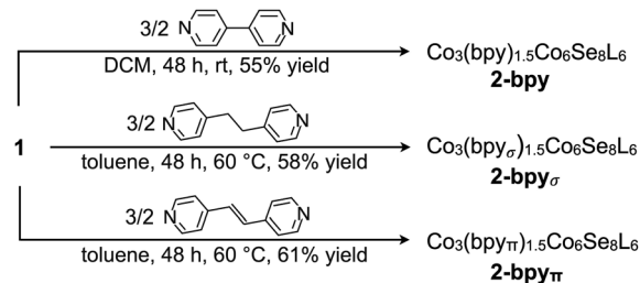
Scheme 2 Self-assembly of van der Waals nanosheets, 2-bpy , 2-bpy}_\pi and 2-bpy}_\sigma , from tritopic nanoblock 1 and pyridyl-based ditopic linkers.
