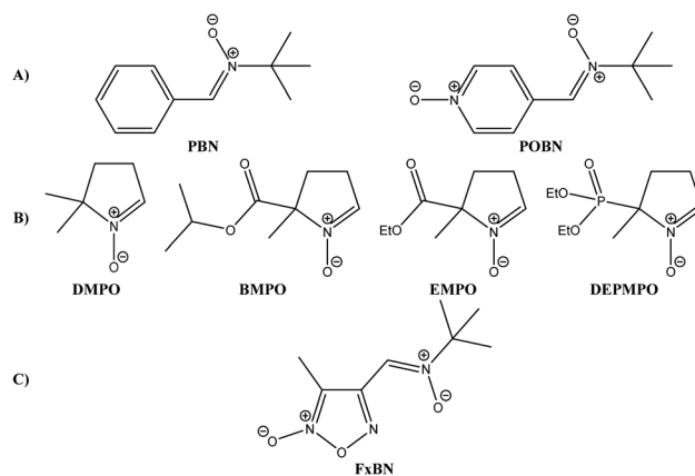
Fig. 1 Structures of most used nitrones as spin trap agents today. (A) PBN and POBN, (B) DMPO, BMPO, EMPO, and DEPMPO, and (C) furoxanyl nitronone (FxBN) described by us.
