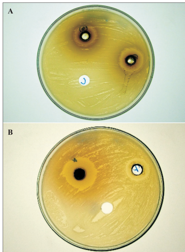
Fig. 1: Antibacterial activity of Vitex negundo Linn. extracts (A) Against Pseudomonas aeruginosa , 5-ethylacetate extract (AI=1.4), 7-ethanol extract (AI=1.2), C-DMSO (AI=0) and (B) against Escherichia coli 2-flowers oil (AI=0.8), 4-petroleum ether extract (AI=1.8), C-DMF (AI=0)
