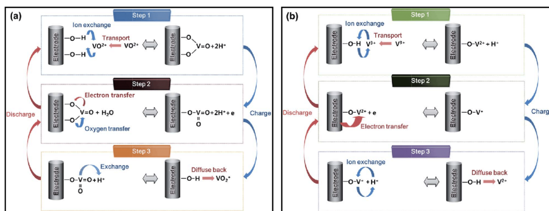
Fig. 12 The redox reaction mechanism proposed by Skyllas-Kazacos for (a) \text{VO}_2^+/\text{VO}^{2+} redox couple in catholyte, (b) the \text{V}^{2+}/\text{V}^{3+} redox couple in VRFB. Reproduced from ref. 31 with permission from Royal Society of Chemistry, copyright 2015.
