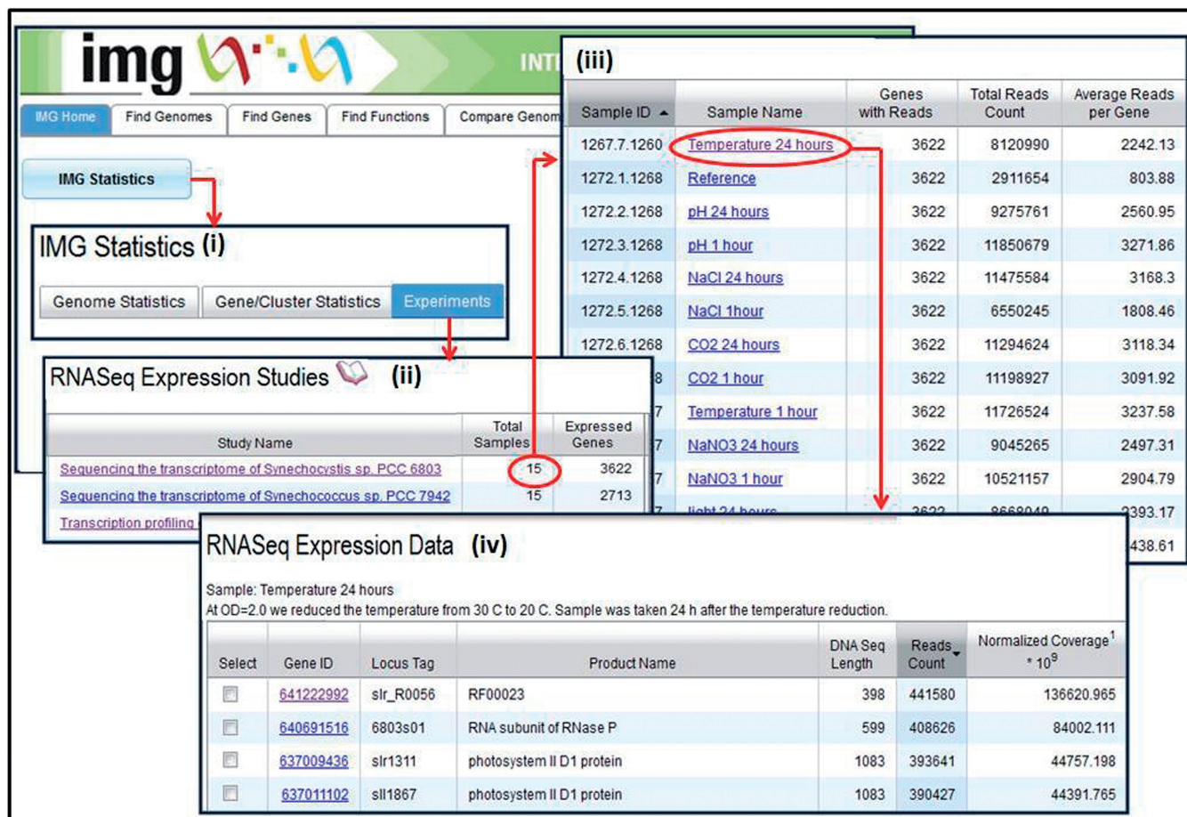
Figure 1. RNA-Seq data organization. (i) 'Omics' datasets generated can be accessed from 'IMG Statistics' on IMG's front page, following the Experiments link available on the 'IMG Statistics' page. (ii) An RNA-Seq study is associated with samples and the number of genes expressed across all samples. (iii) Each sample is associated with the number of expressed genes, the total number of reads and the average number of reads per gene. (iv) An expressed gene is associated with a read count (total number of reads divided by the size of the gene) and normalized coverage (coverage for a gene in the experiment divided by the total number of reads in that experiment).
