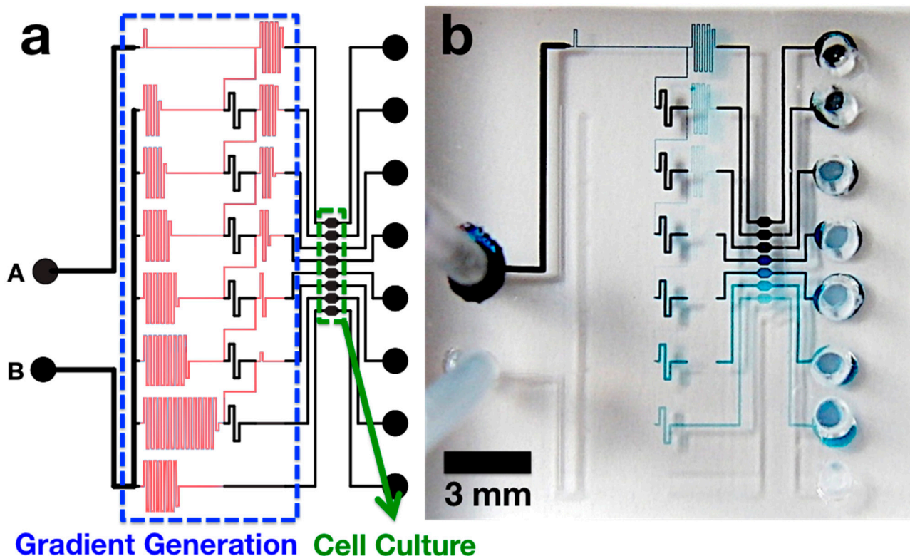
Figure 1. (a) An illustration of microchip design: black and red channels represent 149- \mu\text{m} and 4- \mu\text{m} tall features, respectively; (b) A photograph of the fabricated PDMS chip. Blue food dye solution and water were injected to upper (A) and lower (B) inlet ports, respectively.
