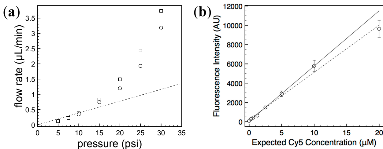
Figure 2. (a) Flow rates achieved by different injection methods: pressure controller ( \square ) and syringe compression ( \circ ). The microchannel used for this measurement had a dimension of 24 \text{ mm} \times 70 \mu\text{m} \times 7 \mu\text{m} ( L \times W \times H ). The dashed line stands for the linear relationship between flow rate ( Q ) and injection pressure ( \Delta P ) expected for a rectangular channel without any deformation: \Delta P = 12 \mu Q L H^{-3} W^{-1} , where \mu is the fluid viscosity of water (assumed to be 0.001 \text{ Pa s} ). The fluidic resistance for the tested channel is 29 \text{ psi min } \mu\text{L}^{-1} . The deviation from the linearity results from deformation of the PDMS channel [20]; (b) Fluorescence intensity measured from each culture chamber after injecting 20 \mu\text{M} Cy5 solution. The error bars stand for standard deviations calculated from 100 \times 100 pixel areas. The linear regression analysis of all 8 data points resulted in y = 489.22 x + 232.17 ( R^2 = 0.991 ; dashed line). The same analysis without the point at the highest concentration produced y = 572.71 x + 51.44 ( R^2 = 0.999 ; solid line).
