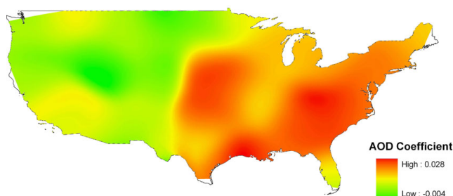
Figure 4 Coefficient raster surface for AOD from geographically weighted regression.
