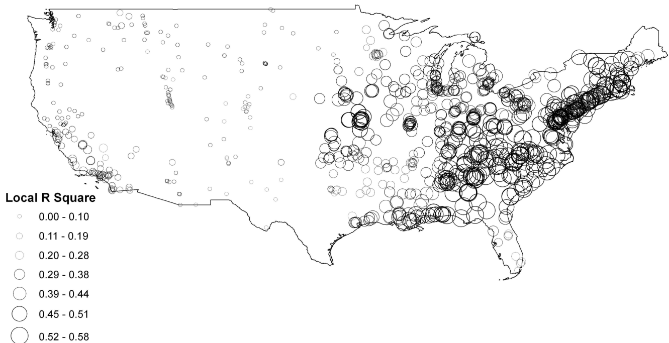
Figure 3 Local R square of geographically weighted regression.
