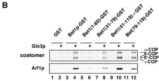
Figure 4. Binding site of COPI on Bet1p-GST. (A) Schematic depiction of Bet1p and GST fusions of Bet1p. (B) The interaction site for Arf1 \Delta N17p and coatomer to Bet1p is comprised within the COOH-terminal 79 amino acids of the cytosolic domain. Although significant amounts were bound to the COOH-terminal 41 amino acids, sequences toward the NH 2 -terminal part may be required and vice versa. Shown are incubations either in the presence of coatomer or Arf1 \Delta N17p with GST fusion proteins of Bet1p. Glo3p was added where indicated. Arf1 \Delta N17p was preincubated with GTP, and GTP was also present during the binding reaction.
