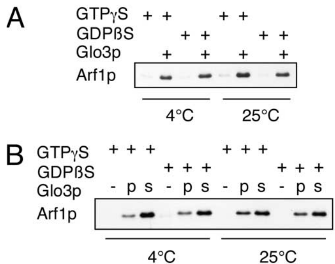
Figure 1. Arf1 \Delta N17p recruitment to membranes is dependent on ARF-GAP. (A) Microsomes from wild-type cells were incubated with Arf1 \Delta N17p, nucleotides, and ARF-GAP (Glo3p) as indicated for 30 min. The Arf1 \Delta N17p that was recruited to the microsomes was separated from the unbound fraction by centrifugation and visualized by immunoblot. (B) The experiment was performed as described in A. Glo3p was only present only during a preincubation step (p) or throughout the recruitment reaction (simultaneous; s).
