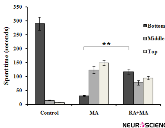
Figure 3. The total time spent by each individual fish from different treatments in the bottom, middle, and top of the one-sided trapezoidal tank
