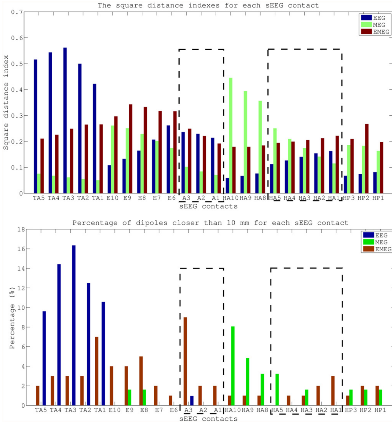
Fig 6. Quantitative comparison of EEG, MEG and EMEG source reconstructions and sEEG contacts. Square distance index and the percentage of dipoles closer than 10 mm for each sEEG contact. The values are given for EEG, MEG and EMEG for subaverages of 10 at -23 ms. The sEEG contacts enclosed by dashed lines are within the seizure onset zone.
