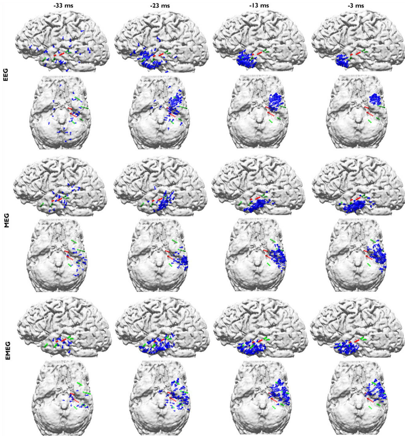
Fig 7. EEG, MEG and EMEG deviation scan peaks of Av10 at different propagation phases. EEG (upper two rows), MEG (middle two rows) and EMEG (lower two rows) deviation scan peaks (illustrated by blue dipoles) of Av10 for time points -33 ms (spike onset, left column) in steps of 10 ms until time point -3 ms (late propagation phase close to EEG peak, right column). Both green and red spheres show the sEEG contacts where frequent interictal activity can be measured, thus giving an impression of the minimal size of the irritative zone, and red spheres alone show seizure onset contacts.
