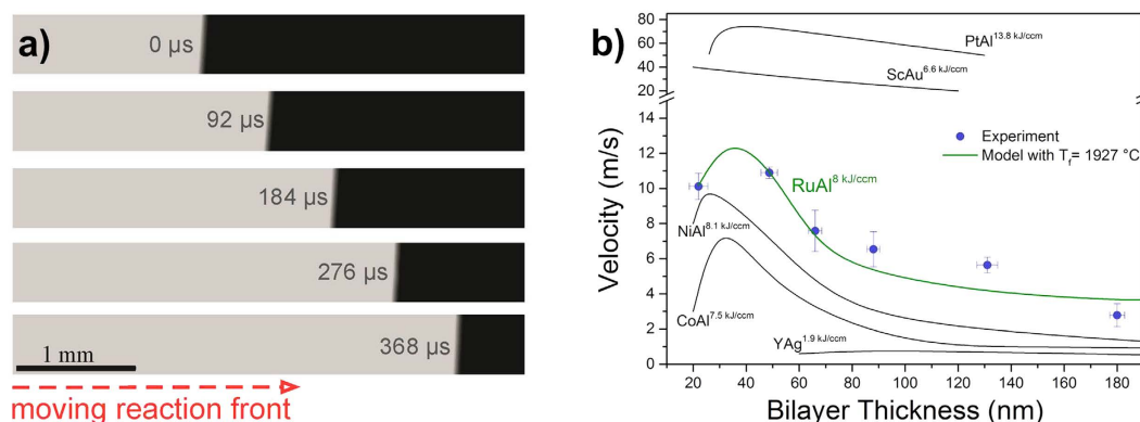
Figure 2. Measured velocities provide evidence for the high energy density stored in Ru/Al multilayers.
