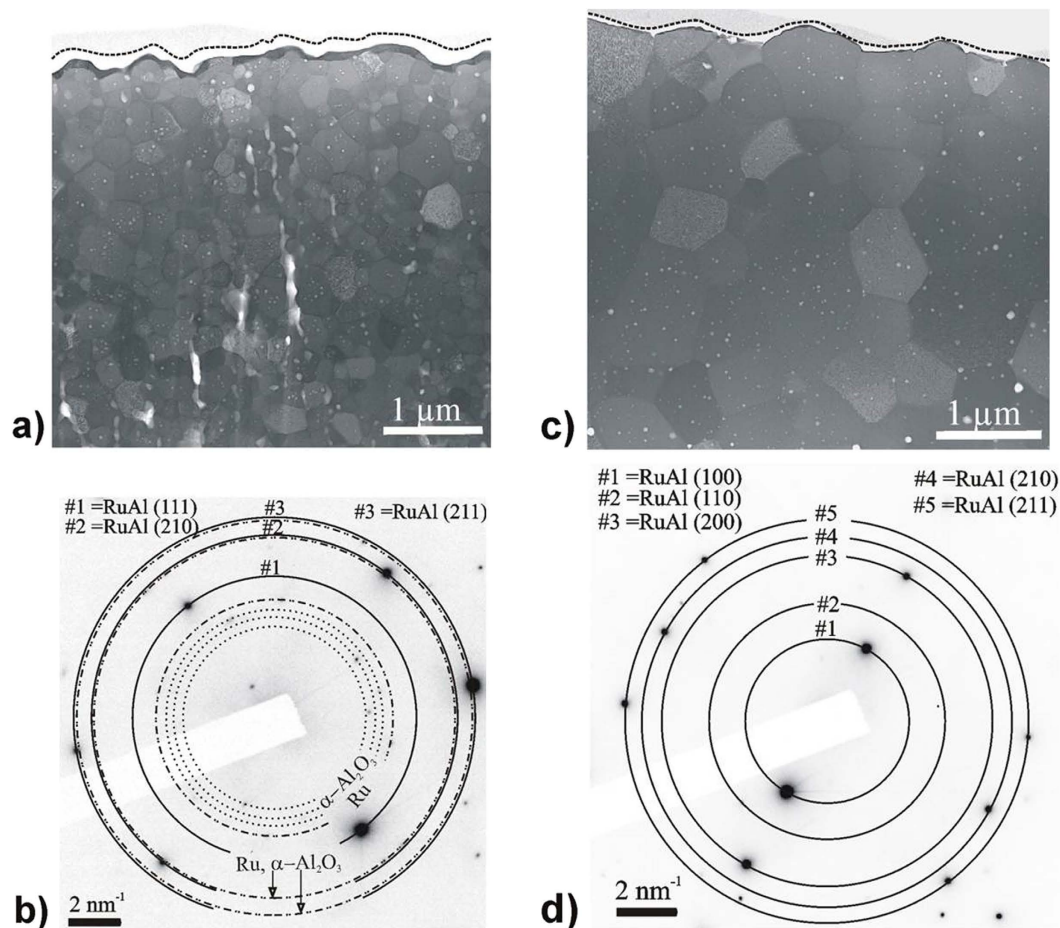
Figure 6. Evidence of single phase, as-reacted foil microstructures as requirement for improved ductility.
