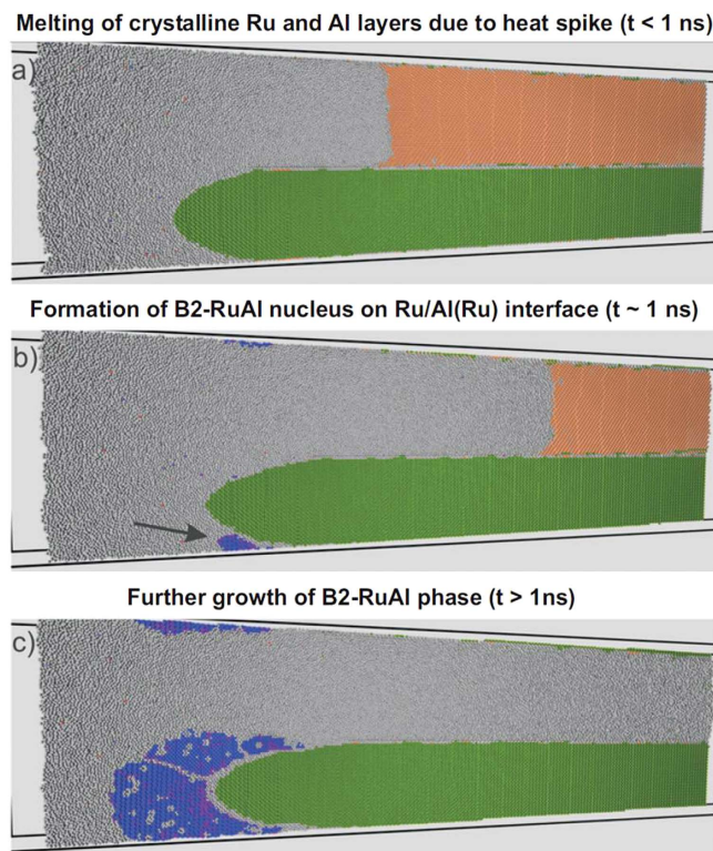
Figure 5. Molecular dynamics simulations of intermixing within Ru/Al multilayers corroborate the transformation behavior to RuAl required for improved ductility. Atoms are colored based on common neighbor analysis: coral atoms have FCC environment; green atoms HCP; blue atoms B2-BCC; purple atoms random-BCC and grey ones are not identified in structure (liquid). (a) The sample after a heat impulse was induced: left part of Ru/Al layers is melted, and then due to heat diffusion, melting of the Al layer happens. (b) A B2-RuAl nucleus forms on the solid Ru - liquid Ru-Al interface. There are few atoms in disordered BCC lattice on the periphery of the nucleus. (c) The growth of the B2-BCC RuAl phase starts from the formed nucleus. We observe quite uniform B2-BCC structure with several inclusions of vacancies (grey spots) and disordered BCC on periphery (purple spots). Full animated MD simulation is attached in the Supplementary.
