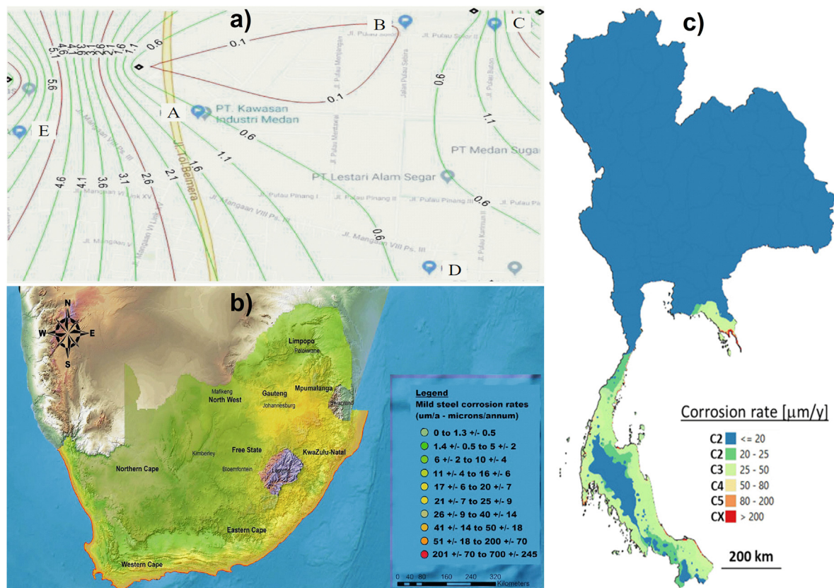
Figure 6. Examples of corrosion maps: (a) isoline map of an industrial area [57], (b) atmospheric corrosion map of South Africa [94], and (c) corrosion rate map of carbon steel (SS400) for tropical climate in Thailand [129].
