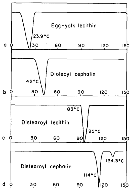
FIGURE 1 D.T.A. curves of pure phospholipids, showing the major endothermic peaks for the following: a , Egg yolk lecithin. b , 2,3-dioleoyl-DL-phosphatidyl-ethanolamine. c , 2,3-distearoyl-DL-phosphatidyl-choline. d , 2,3-distearoyl-DL-phosphatidyl-ethanolamine.
