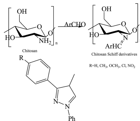
Scheme 17 Synthesis of chitosan Schiff bases (ChBs).
