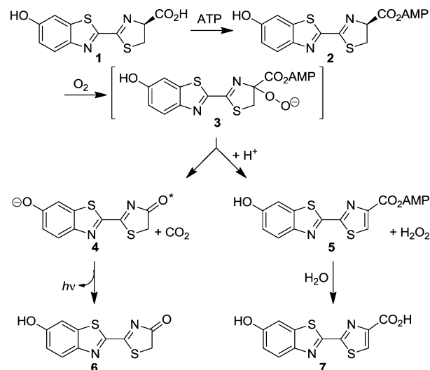
Scheme 1. Accepted pathway of firefly bioluminescence.
