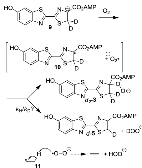
Scheme 3. Alternative reaction pathways for the enolate of luciferyl adenylate.
