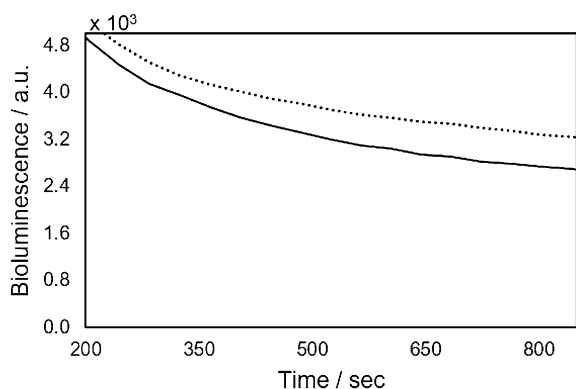
Figure 1. Time course of bioluminescence decay at late reaction times for 1 (solid) and d_2 - 1 (dashed).
