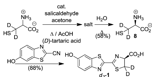
Scheme 2. Synthesis of d_2 -luciferin.
