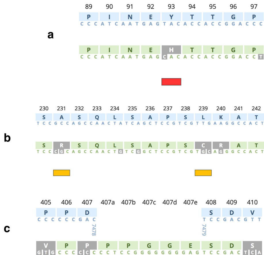
Fig. 6 Genome visualisation of the NS5A viral protein within a subtype 3a query sequence via the HCV-GLUE web report. The submitted query sequence in green is contrasted with a user-selected reference sequence in blue. Differences between the query and reference are highlighted in inverted grey. In a the 93H RAS is highlighted by a red annotation bar and is shown to have arisen from a single nucleotide change relative to the subtype 3a reference (NC_009824) in the first nucleotide position within the codon. In b the query sequence contains amino-acid differences relative to the subtype 3a reference sequence at positions 231, 239 and 240. There are nucleotide differences within codons 234 and 235 but these are synonymous. The amino acid differences at 231 and 239 are atypical for subtype 3a as indicated by the yellow annotation bars, whereas the Arginine (R) at position 240 is typical for the subtype. In c the subtype 3a query sequence is shown alongside the HCV master reference (NC_004102); an insertion of 5 amino acids in the query sequence between codon locations 407 and 408 is shown; the consecutive nucleotide positions 7478 and 7479 in the master reference are also given to clarify the insertion
