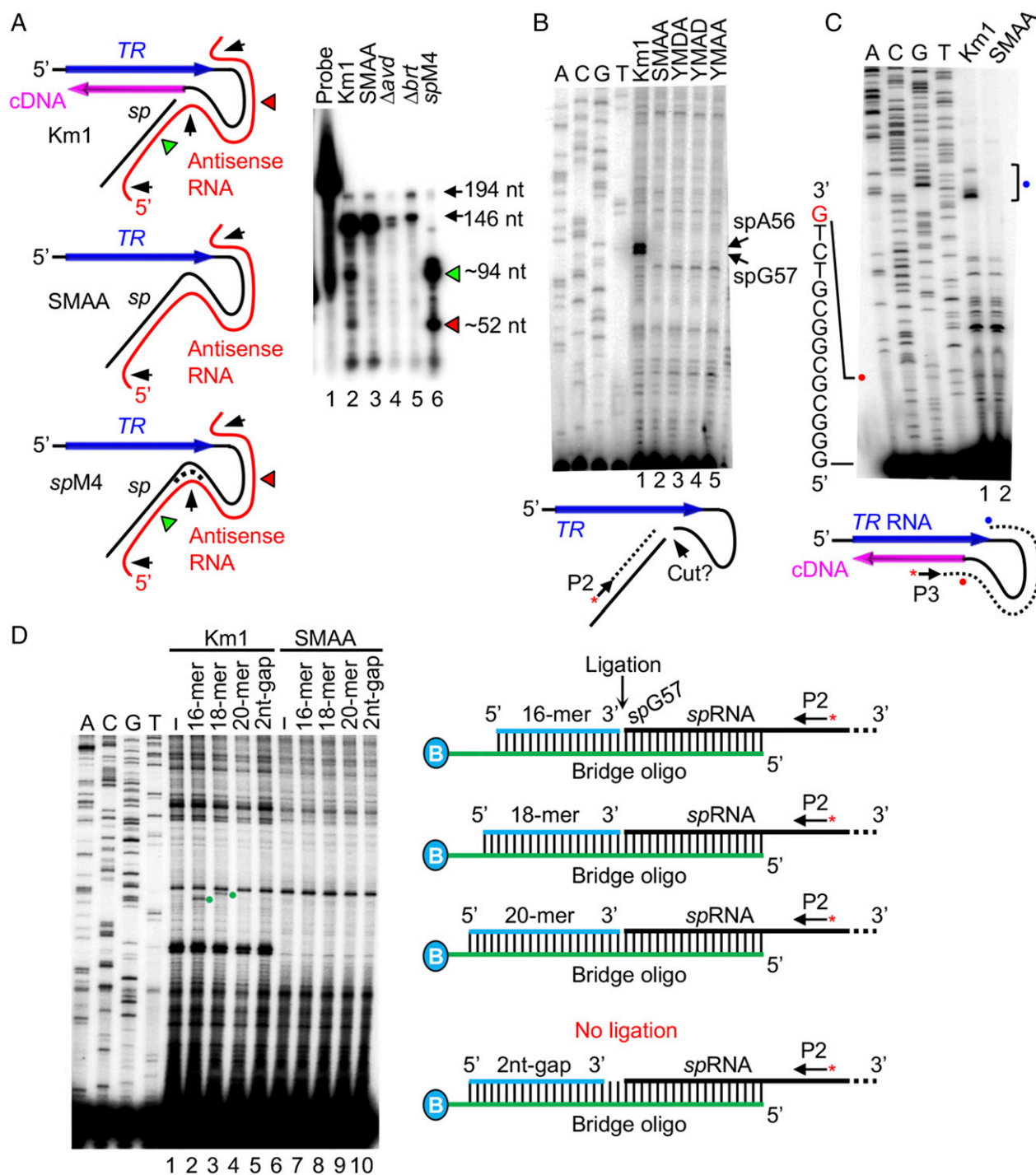
Fig. 4. bRT-dependent TR RNA cleavage at the cDNA priming site. ( A , Left ) Diagram of the RNase protection assay. TR , blue; sp , black; cDNA, pink; uniformly labeled antisense RNA probe, red. Arrowheads indicate RNase cleavage sites ( Right ). spM4 , which has four mutated residues at the priming area, served as a positive control. The two protected fragments are indicated by green and red triangles. Km1 and SMAA are wild-type and catalytically inactive bRT constructs, respectively. ( A , Right ) RNase protection analysis. The 194-nt band is probe, the 146-nt band is probe cleaved by RNase at the unpaired ends, and the 94- and 52-nt bands are RNase protection products resulting from cleavage at the priming region and the two ends. \Delta avd and \Delta brt are deletion mutants of avd and brt , respectively. ( B ) Primer extension assay of wild type ( Km1 ) and bRT-deficient mutants ( SMAA , YMDA , YMAD and YMAA ) with a ^{32} P-labeled primer ( P2 ) annealing downstream of spA56 . Two bRT-dependent bands ( spA56 and spG57 ) are observed, suggesting that TR RNA is either cleaved or branched at spA56 . Sequencing ladders were generated from pMX- Km1 with the same labeled primer. Shown below is a diagram of TR RNA cleavage at spA56 . ( C ) Primer extension assay of Km1 and the SMAA mutant with a ^{32} P-labeled primer ( P3 ) annealing to (-) cDNA. Km1 -specific terminations were detected in the IMH* region (blue dot) after passing the cDNA-RNA primer junction (red dot). The junction did not block primer extension. Sequencing ladders were generated from pMX- Km1 with the same labeled primer. ( D ) Primer extension of splint ligation products with ^{32} P-labeled primer P2 . Ligation of adaptor DNA oligos to spG57 of cleaved spRNA occurred in the presence of a Bridge DNA oligo (3' biotin-tagged) and T4 DNA ligase. 16-mer, 18-mer, and 20-mer are 16-nt, 18-nt, and 20-nt adaptors. Oligo 2nt-gap is 2 nt away from spG57 after annealing. -, a negative control with no adaptor oligo added. Sequencing ladders were generated as in B . Primer extension products generated from those of splint ligation are marked by green dots. The ligation product of the 20-mer adaptor could not be detected because of a comigrating background band.
