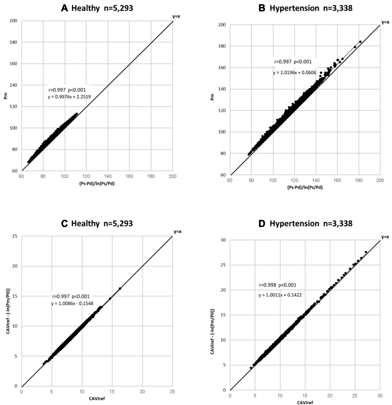
Figure 5 Relationship between \frac{Ps-Pd}{\ln(Ps)-\ln(Pd)} and Pm for healthy group (A) and hypertensive group (B) analyzed with the data from Shirai et al. 21 Relationship between CAVIref and CAVIref - (-\ln(\frac{Pm}{P0})) for healthy group (C) and hypertensive group (D) analyzed with the data from Shirai et al. 21 Abbreviations: Ps, systolic blood pressure; Pd, diastolic blood pressure; Pm, mid-pressure; CAVIref, cardio-ankle vascular index (CAVI) with reference blood pressure; P 0 , reference blood pressure.
