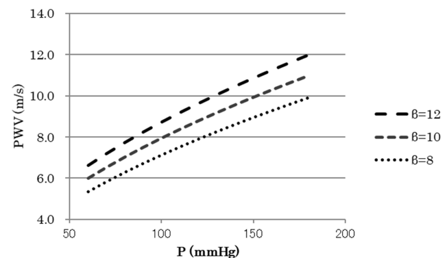
Figure 1 Relationship between P and PWV in Equation 1.
