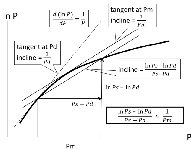
Figure 4 Schematics to show \frac{\ln(P_s) - \ln(P_d)}{P_s - P_d} \approx \frac{1}{P_m} . Abbreviations: P, blood pressure; P_s , systolic blood pressure; P_d , diastolic blood pressure; P_m , mid-pressure.
