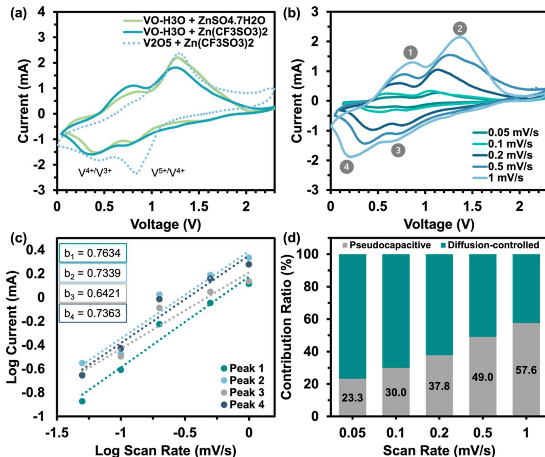
Fig. 3 Cyclic voltammograms of (a) VO-H 3 O and reagent V 2 O 5 in cells against Zn/Zn 2+ in two aqueous electrolytes, 3 M ZnSO 4 ·7H 2 O and 3 M Zn(CF 3 SO 3 ) 2 , at a scan rate of 0.5 mV s -1 and (b) VO-H 3 O in 3 M Zn(CF 3 SO 3 ) 2 at varied scan rates (0.05 to 1 mV s -1 ). (c) Plot of log current against log scan rate showing the b -values of the four peaks. (d) Contribution ratio of pseudocapacitive and diffusion-controlled behaviors at increasing scan rates.
