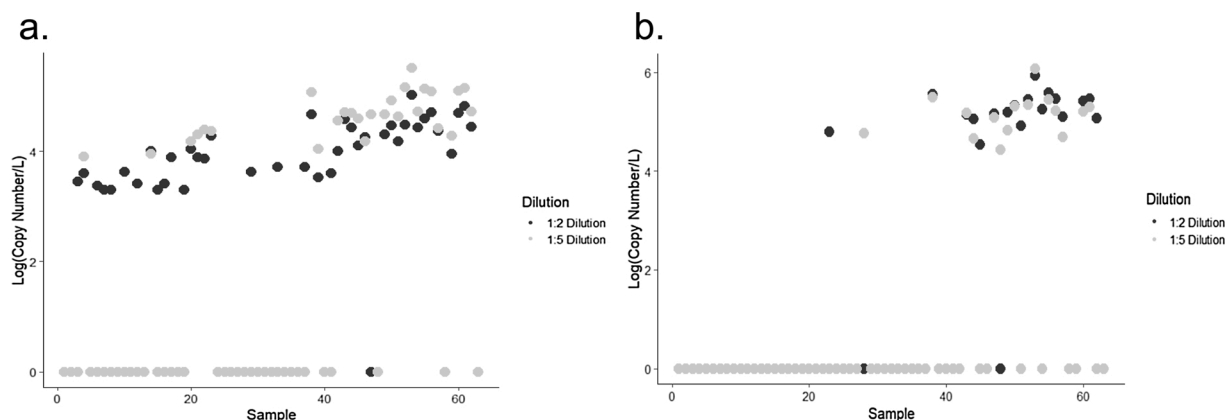
Fig. 1. Effect of Dilution on Detection of SARS-CoV-2 RNA in Wastewater: Extracts had been diluted at both a 1:2 (black dots) and 1:5 dilution (grey dots) in AE buffer prior to reverse transcription and PCR amplification and samples were analyzed using both (a) RT-ddPCR and (b) RT-qPCR by the processing group based out of IMS.
