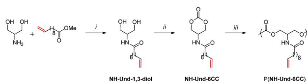
Fig. 1 Synthesis of lipidic polycarbonate from methyl undecenoate and 2-amino-1,3-propanediol.
