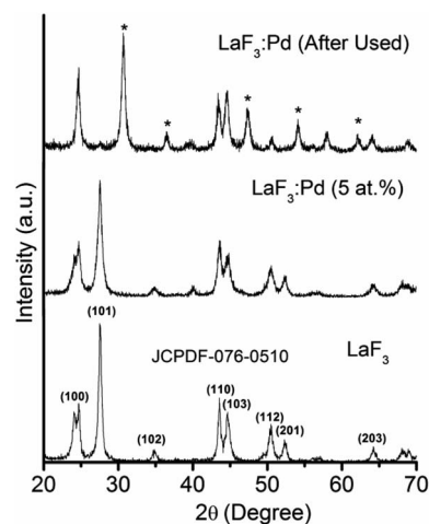
Fig. 2 XRD pattern of LaF 3 ·Pd.
