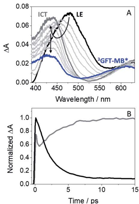
Fig. 3 (A) Femtosecond transient absorption spectra from 0.5 ps (black) to 2 ns (blue) for GFT-MB. (B) Kinetic traces monitored at 480 nm (black) and 435 nm (dark gray). Measurements were performed in acetonitrile after excitation at 330 nm.
