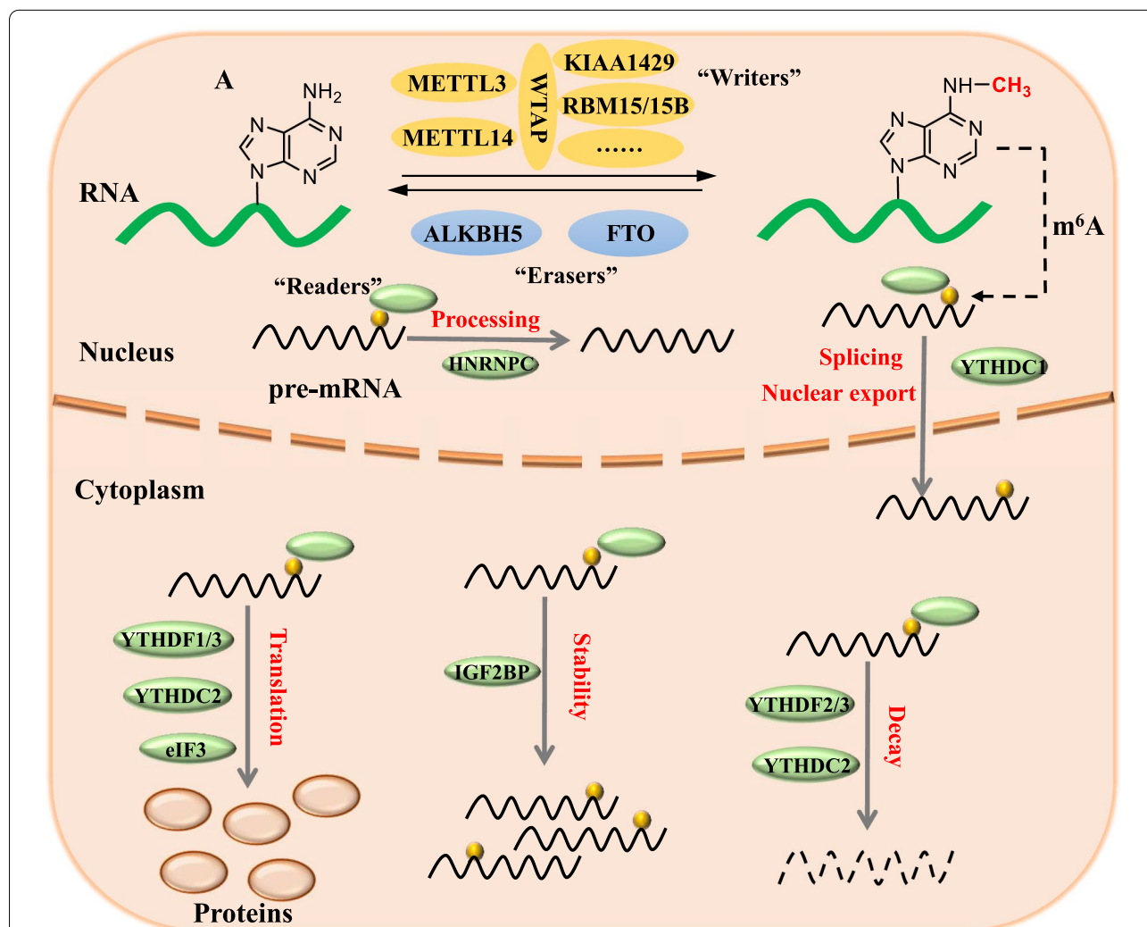
Fig. 2 The dynamic and reversible m 6 A RNA modification and its role in RNA metabolism. m 6 A RNA methylation is exerted by methyltransferases (METTL3, METTL14, WTAP, etc.), removed by demethylases (FTO and ALKBH5). mRNA processing, splicing, stability, translation, and subcellular localization can be influenced by m 6 A modification through the actions of m 6 A binding proteins
