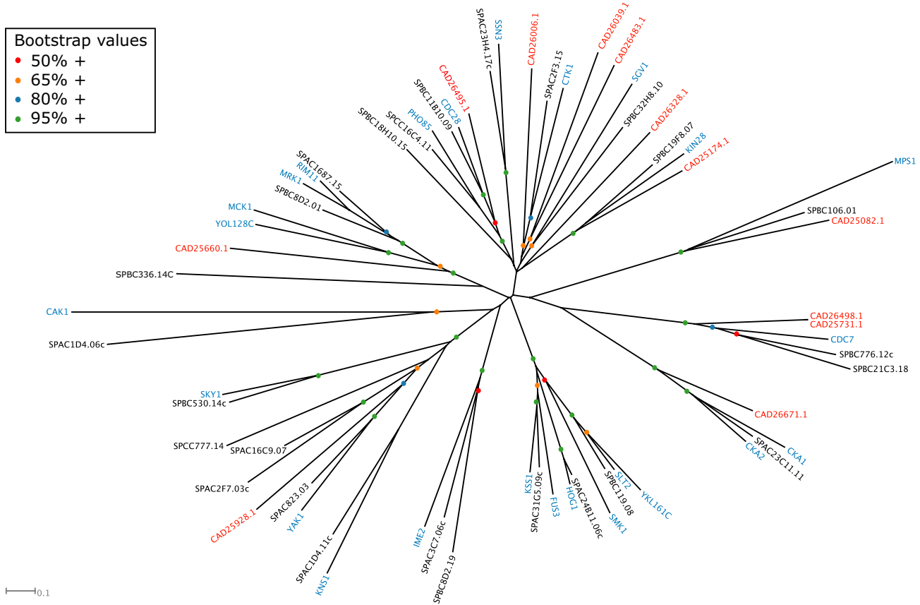
Figure 4 Unrooted tree of the CMGC kinases of S. cerevisiae (blue), S. pombe (black) and E. cucuculi (red).
