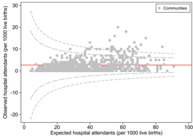
Fig. 2. Funnel plot of health facility attendants of sick children in Nigeria, 2013. The red line represents the mean line while the inner dotted lines are 95% confidence intervals and outer dotted lines are 99.9% confidence intervals derived using the Poisson distribution.
