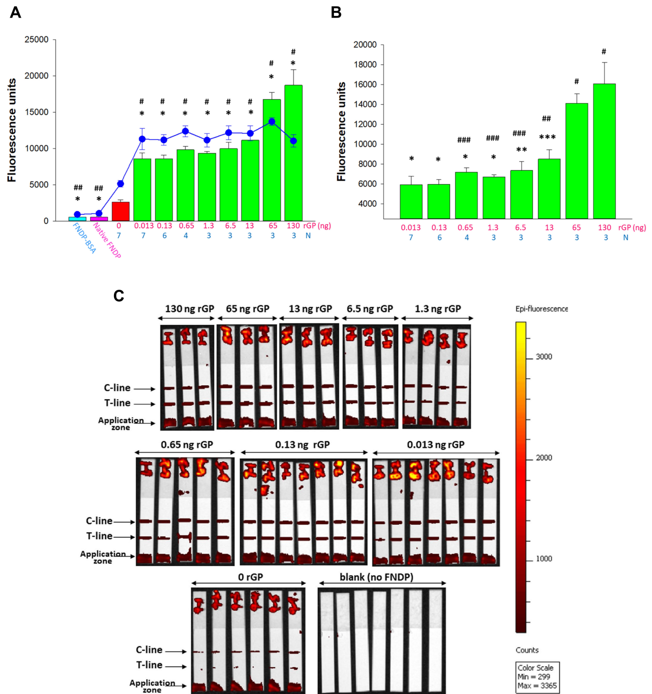
Figure 10 Sensitivity of FNDP-NV-200nm-c13C6-rGP detection in human serum (depleted of IgG) using an AX-2X-S OED. Notes: (A) Fluorescence intensity of the test line (bar graph) and control line (blue line). Error bars represent SD from the number of replicates indicated by the blue number below each mass of rGP mass (pink numbers). Test Line: (*) P<0.001 and Control Line (##) P<0.001, (###) P=0.003 were calculated using One-way ANOVA for difference between strips run with FNDP-NV-200nm-c13C6 and with FNDP-NV-200nm-c13C6-rGP. (B) Fluorescence intensity of T-line for various amounts of rGP (indicated by pink numbers) deducted by background of FNDP-NV-200nm-c13C6 (rGP = 0 ng). (*) P<0.001, (**) P = 0.003, (***) P = 0.005 were calculated using One-way ANOVA for difference between strips run with the highest (130 ng) amount of rGP. (#) P<0.001, (##) P = 0.003, (###) P<0.05 were calculated using One-way ANOVA for difference between strips run with the lowest (0.013 ng) amount of rGP. (C) IVIS-50 images of test strips. Abbreviations: FNDP-NV-200nm-c13C6, fluorescent nanodiamond particles with NV active centers, 200 nm diameter, coupled to chimeric c13C6 monoclonal antibody; rGP, recombinant glycoprotein; mAb, monoclonal antibody; SD, standard deviation; N, number of strips per sample; ng, nanograms.
