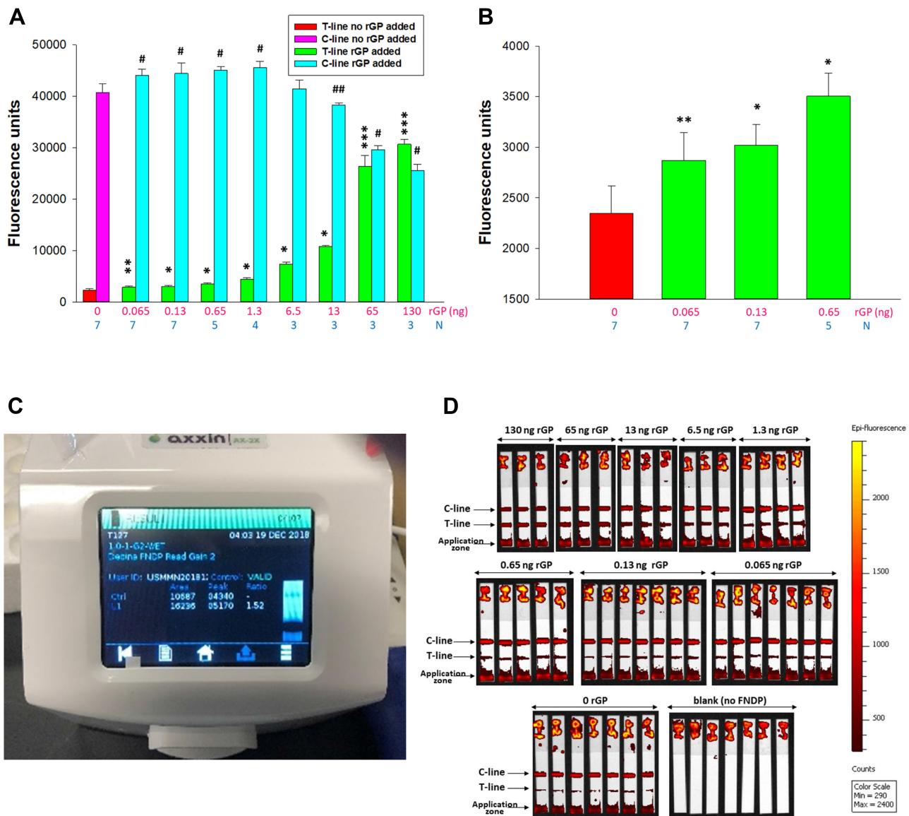
Figure 9 Sensitivity of FNNDP-NV-200nm-c13C6-rGP detection using an AX-2X-S OED.
