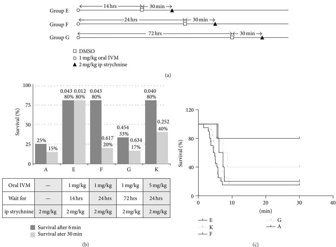
FIGURE 2: Protection against strychnine toxicity by oral ivermectin. (a) Dosage schedule for oral IVM administration. Groups E–G received 1 mg/kg IVM in DMSO (open circles), followed by vehicle injection (DMSO, open squares) after the indicated waiting time, and injection of 2 mg/kg strychnine (solid triangles) after another 30 min. Number of animals: E ( n = 5 ); F ( n = 5 ); G ( n = 12 ). (b) Survival rates of groups A–D. The P values for statistical significance (Fisher's one-tailed t -test), relative to control (group A), are given above each column. (c) Time course of survival in groups E–G. Survival curve for control group A (Figure 1(c)), receiving strychnine only, is added.
