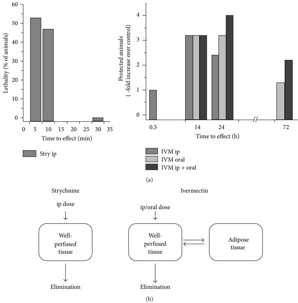
FIGURE 4: Time course of strychnine and ivermectin effects. (a) Time course of strychnine and ivermectin action. For strychnine, lethality (% of animals) within 0–5 and 5–10 min is plotted. After 30 min, no effects of strychnine were observed. For ivermectin, the -fold increase in survival time >6 min was plotted relative to control animals which received only vehicle. (b) One- and two-compartment models of distribution of strychnine and ivermectin in tissue.
