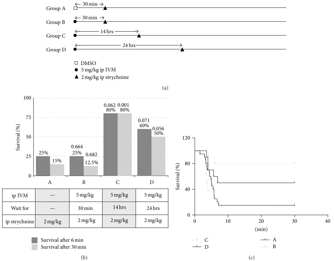
FIGURE 1: Protection against strychnine toxicity by intraperitoneal ivermectin. (a) Dosage schedule for systemic IVM administration. Group A received vehicle (DMSO, open square), groups B–D received 5 mg/kg IVM (solid circles), followed by 2 mg/kg strychnine (solid triangles) after the indicated waiting period. Number of animals: A ( n = 20); B ( n = 8); C ( n = 10); D ( n = 10). (b) Survival rates of groups A–D. The P values for statistical significance (Fisher’s one-tailed t -test), relative to control (group A) are given above each column. (c) Time course of survival in groups A–D.
