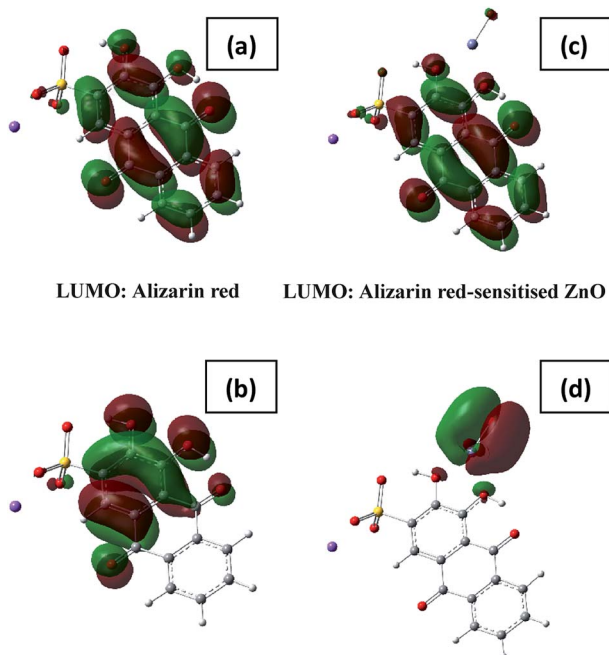
Fig. 8 HOMO and LUMO orbitals of alizarin red and the likely structure of the alizarin red-sensitised ZnO. A key feature of the molecular orbitals is the migration of the HOMO from the dye to the ZnO, this neatly illustrates the mixing of the molecular orbitals. The HOMO–LUMO energy gaps measure 5.65 and 2.77 eV, respectively. HOMO and LUMO states of alizarin red and alizarin red-sensitised ZnO species.
