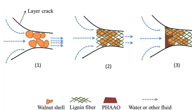
Fig. 13 Mechanism of plugging process.
