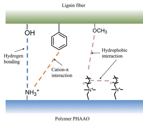
Fig. 18 Interaction forces between lignin fiber and polymer.
