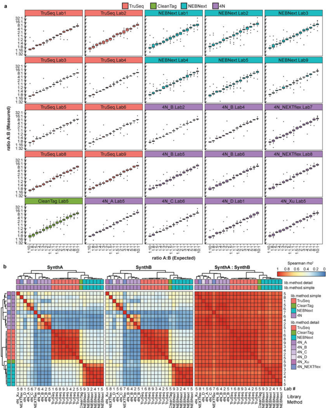
Figure 3. Small RNA-seq accuracy and cross-protocol concordance in measuring relative expression levels between samples
