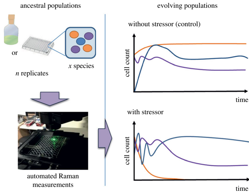
Figure 2. Perspective of microbial experimental evolution using Raman spectroscopy. Long-term cultures composed of single or multiple species are evolved in the presence or absence of varying levels of stressors. Population dynamics monitoring, as well as the characterization and isolation of emerging phenotypes (e.g. antibiotic-resistant mutants), could be performed by Raman spectral analysis, given the condition they exhibit different spectral markers (a specific pigment, amino acids, etc.), as suggested by recent studies [7–9].
