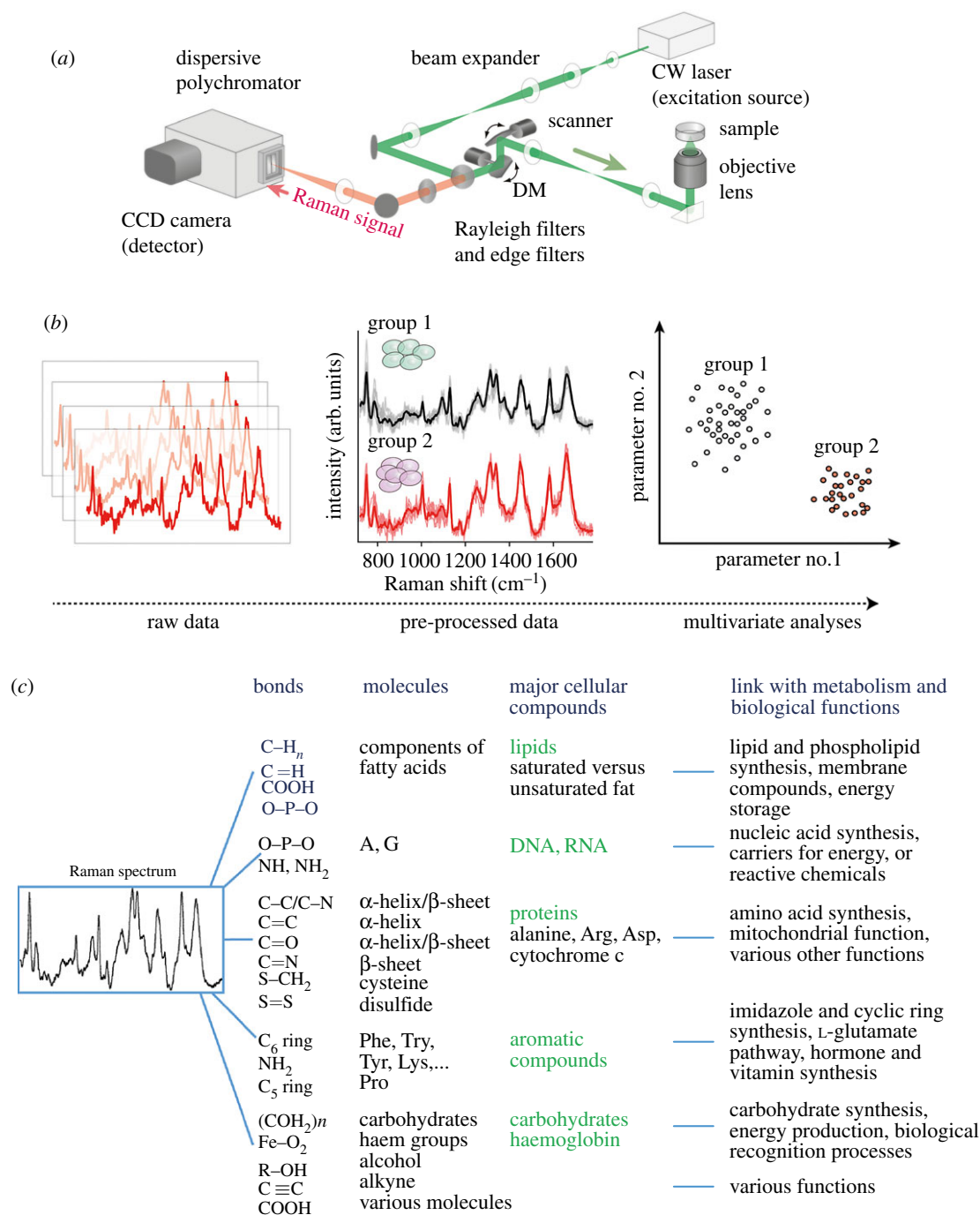
Figure 1. A general overview of Raman spectroscopy. (a) A generalized overview of the optical set-up for a typical spontaneous Raman spectroscopic microscope. A monochromatic laser light illuminates the sample, emitting Raman scattering light. A small portion of this scattering passes through the objective lens and goes through the optical pathway to the dispersive polychromator (i.e. spectrophotometer), where it is captured by a CCD detector. (b) Raw spectral data must be processed through various procedures to improve the quality of the signal by removing noise (e.g. due to cosmic rays, the auto-fluorescence signal of the samples or from unavoidable technical variations). Because spectra are not always useful to visualize and are characterized by the molecular composition between each group or conditions, they are usually used as the input for multi-variate analyses such as principal component analyses, projection latent structure analyses, discriminant analyses and support vector machines, which are particularly powerful for identifying and discriminating individuals from the contribution of all or specific Raman wavelengths. (c) Representation of the inherent layers that contribute to the complex spectral signature.
