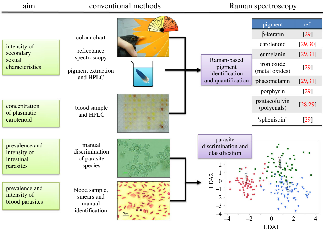
Figure 3. Example of the advantages of Raman spectroscopy in evaluating the effects of food availability and parasitism on the secondary sexual characteristics in birds. In black birds, carotenoid pigments are an indicator of good health as their concentration is directly correlated with food availability and the immuno-resistance against parasitism [32]. Raman spectroscopy is known to provide specific signatures for pigment identification and quantification, as shown in the pioneering work of Thomas et al. [29,30], Galvan & Jorge [31] and Fernandes et al. [28], thus giving an alternative to the destructive and time-consuming conventional methods currently used by ecologists. This may become useful to monitor indirectly the health status of birds in natural populations. Likewise, the discrimination of intestinal and blood parasite species (copepoda, protozoa, etc.) could be done by spectral measurements in a systematic manner without the need for smears and hazardous manual identification. We show here a hypothetical example of linear discriminant analysis (LDA), in which three groups are identified (each point of the plot corresponds to a spectrum taken from one individual).
