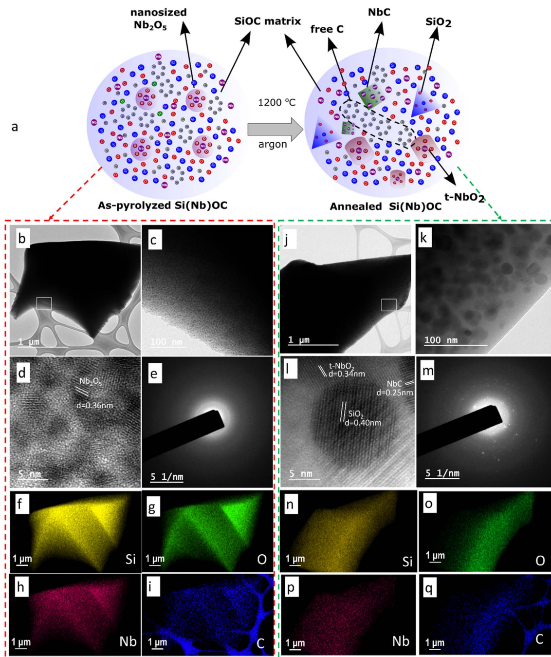
Fig. 3 (a) Schematic representation of fabrication process of Si(Nb)OC composites, (b) and (c) TEM microstructures, (d) high resolution microstructure reveals lattice fringes of ordered nano \text{Nb}_2\text{O}_5 in amorphous SiOC matrix, (e) SAED diffraction pattern shows amorphous nature of as-pyrolyzed Si(Nb)OC composite, (f–i) elemental mapping of as-pyrolyzed Si(Nb)OC composite shows the presence and uniform distribution of elements Si, O, Nb & C; (j) and (k) TEM microstructures of annealed Si(Nb)OC, (l) high resolution microstructure reveals lattice fringes of t\text{-NbO}_2 , NbC and \text{SiO}_2 nanocrystals in amorphous SiOC matrix, (m) SAED diffraction pattern shows polycrystalline nature of annealed Si(Nb)OC composite, (n–q) elemental mapping of annealed Si(Nb)OC composite shows the presence and uniform distribution of elements Si, O, Nb & segregated C.
